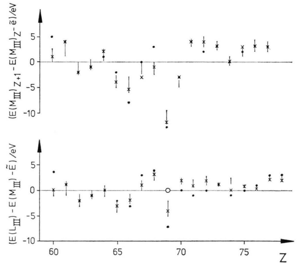
Fig. 2. Deviations of the tabulated distances E(L_{III}) - E(M_{III}) from the approximate energy difference \tilde{E} and of the tabulated differences E(M_{III})_{Z+1} - E(M_{III})_Z from the approximate energy difference \tilde{e} for 60 \leq Z \leq 78 . The data of Hagström et al. ^2 are marked \bullet , those of Lederer et al. ^3 are given by \times and the values of Bearden and Burr ^4 by the vertical line whose length corresponds with the quoted error. The open circle is the result of the present experiment.
