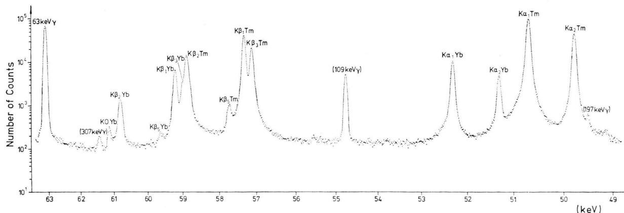
Fig. 1. Spectrum of the K-Röntgen lines emitted from a ^{169}Yb source and measured in the first order of reflection.
